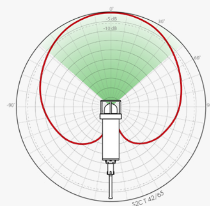
Transducer directivity pattern
